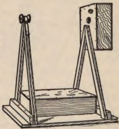
FIG. 149. — Standard for the Ferris Wheel.
